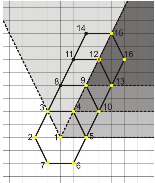
Fig.2 Directional Hexagon-based search pattern
