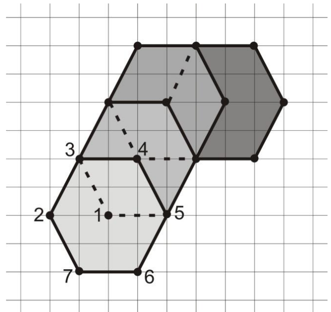
Fig.1. Hexagonal coarse search
