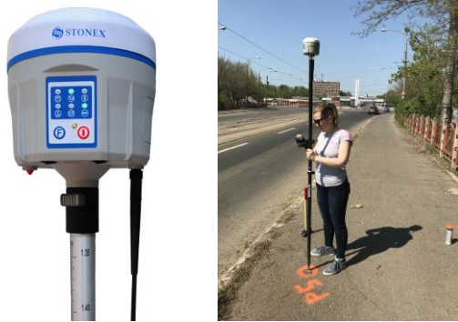
Figure 7 a) GPS RTK Stonex S10 b) GPS RTK Stonex S10 with accessories
