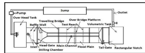
Figure 1. Schematic drawing of whole experimental tilting flume
