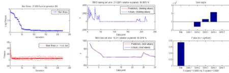
Figure 9. Plot for Fitness, Prediction along with Bias and Gene for data set V in GP
