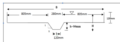
Figure 2. Straight Compound Channel Section
