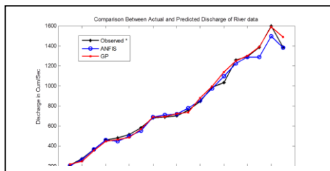
Figure 13. Predicted discharge using GP and ANFIS of Data Set IV
