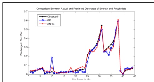
Figure 12. Predicted discharge using GP and ANFIS for Data Set III
