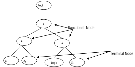
Figure 4. GP Tree for expression ax_1 + \text{Log } b x_2
