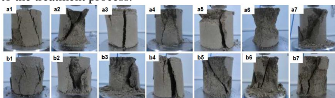
Figure8. The development of the studied samples behavior from ductile (for untreated compacted samples) to brittle (for stabilized samples); a) EB; a1) Natural Compacted EB; a2) EB+CKD 7days; a3) EB+CKD 28days; a4) EB+CKD 90days; a5) EB+L/CKD 7days; a6) EB+L/CKD 28days; a7) EB+L/CKD 90days; b) EQ; d1) Natural Compacted EQ; b2) EQ +CKD 7days; b3) EQ +CKD 28days; b4) EQ +CKD 90days; b5) EQ +L/CK 7days; b6) EQ +L/CKD 28days; b7) EQ +L/CKD 90days
