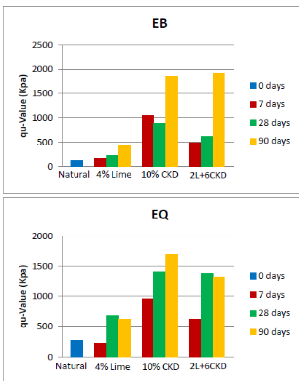
Figure7. Unconfined compressive strength values of the studied samples value from 276.67Kpa to 624.01, 1696.97, and 1315.77Kpa, respectively. Figure 8 showed the development of behavior of the studied Esna shale samples from ductile to brittle due to the treatment process.
