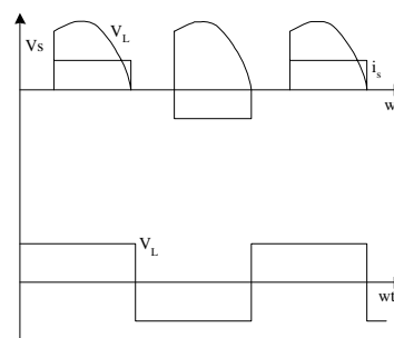
Fig. 1: Waveforms for a) Output Voltage & input current for a single phase Converter b) Output Voltage of a single phase inverter
