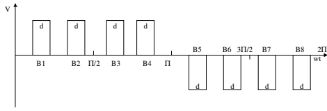
Fig. 2: Modulated Voltage Waveform for Selective Harmonic Elimination
