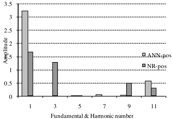
Fig.7: Comparison of Fundamental & other harmonic voltages
