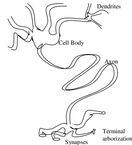
Fig. 3: Biological Neuron
