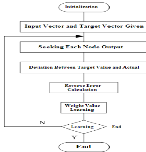
Fig. 2 Flowchart for ANN Training
