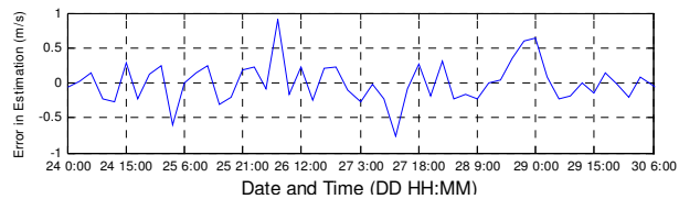
Fig. 6 Fall Season, 24 October, 2010 to 30 October, 2010: a) actual wind speed, solid line, together with the forecasted wind speed, dashed line, in m/s b) Error in estimation, in m/s
