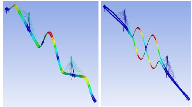
Figure 4.4. 3 rd Vertical bending
