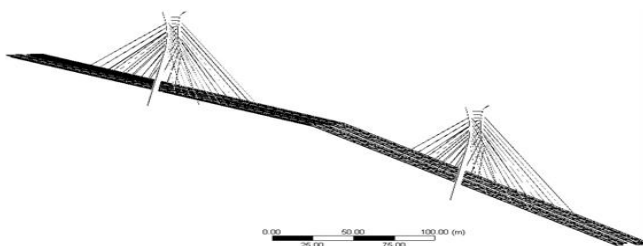
Figure 3.4. Side View of discretized Lekki Bridge
