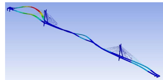
Figure 4.7. 4 th Vertical bending
