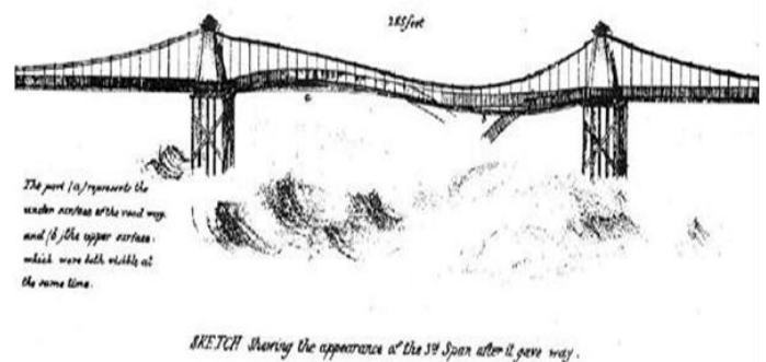
Figure 1.1. Fatal undulating motion of the third span of the Brighton Chain Pier in the storm of 1836 sketched by Reid (J.S. Russell, 1839)
