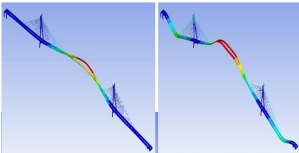
Figure 4.2. 1 st Vertical bending
