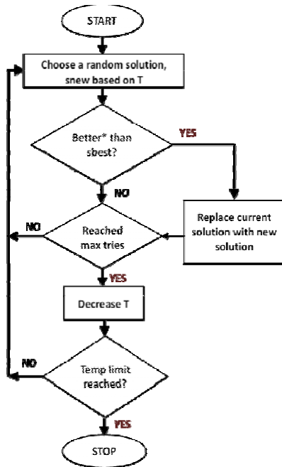
Figure 2. Flowchart of Simulated Annealing.
