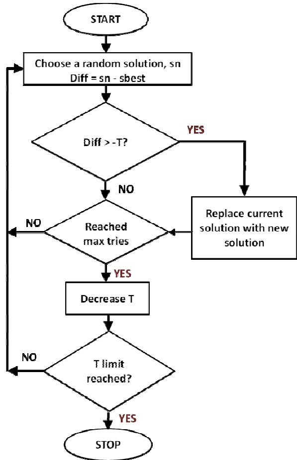
Figure 3. Flowchart of Threshold Accepting.
