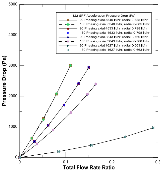
Fig.2 Acceleration pressure drop in 122 SPF 90° And 180° phasing
