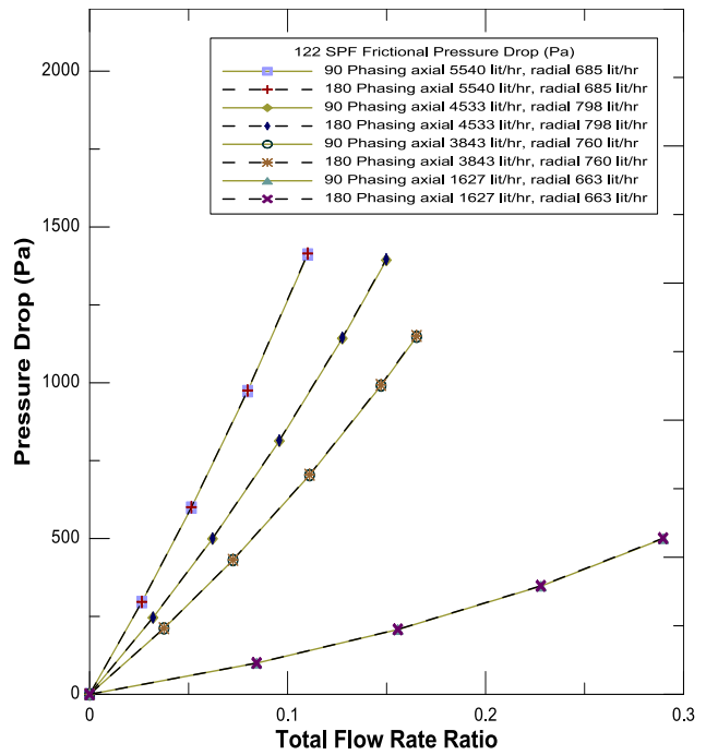
Fig.3 Frictional pressure drop in 122 SPF 90° and 180° phasing
