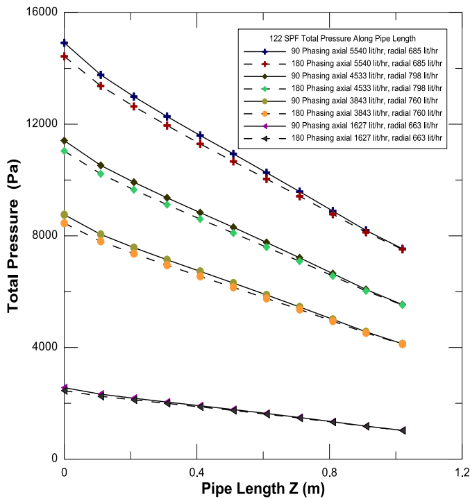
Fig.5 Total pressure along pipe length
