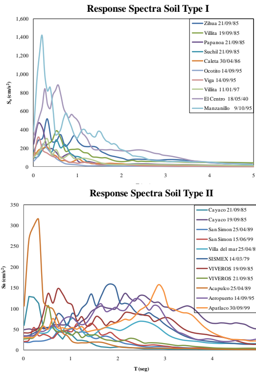
Figure 3. Pseudoacceleration response spectra for soils types I and II
