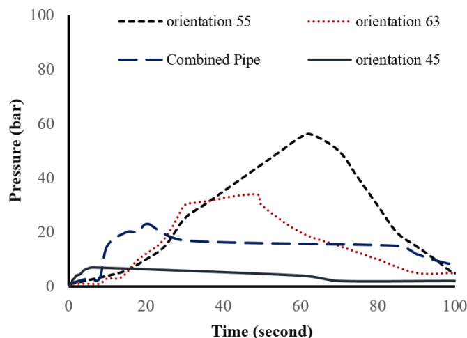
Figure 2. Loading history of the four pipes with different fillament angles.
