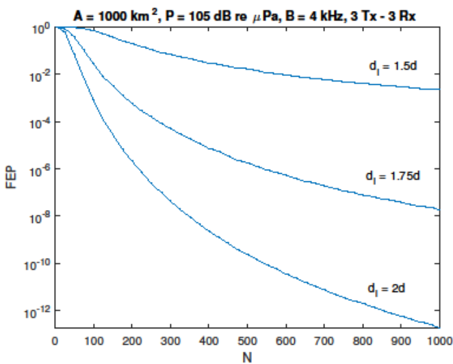
Fig. 6. Average route FEP for 3 \times 3 MIMO AUV-to-AUV links for various interferer distances.
