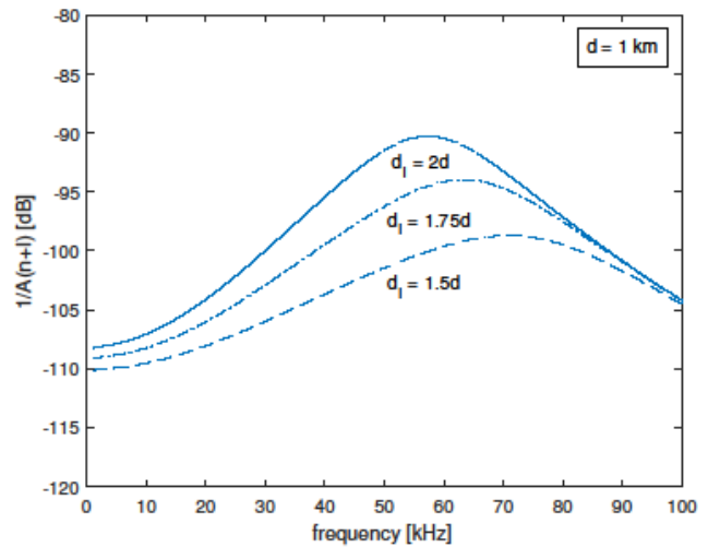
Fig. 1. SINR for d = 1 km.
