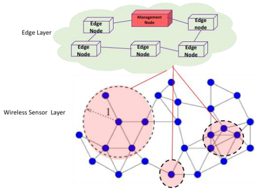
Figure 2. Edge with DLT based on proximity-Context
