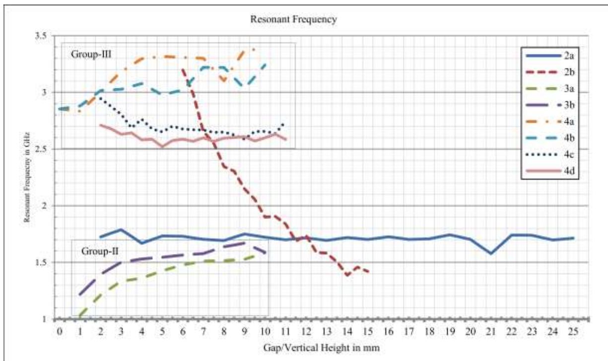
Figure 5 – Resonant frequencies for various configurations of SRs combined.
