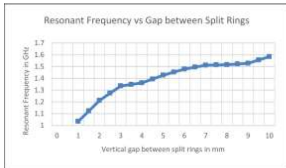
Figure 3a. Lower SR placed 10 mm above the base of cavity (one third of cavity height) and gap varied from 1 mm to 10 mm
