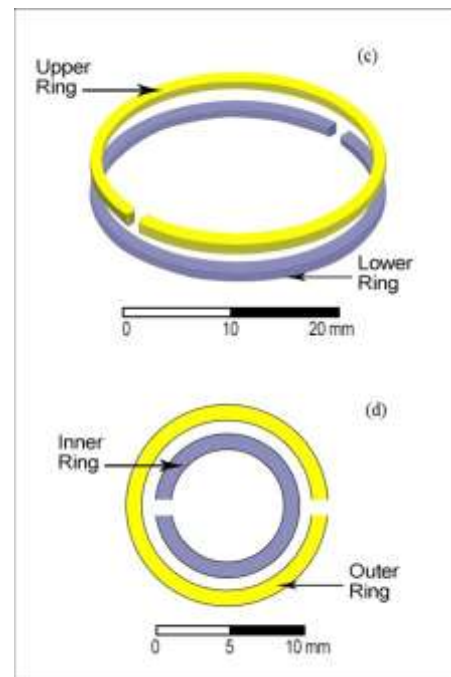
Figure 3 (c) HFSS 3-D model of VS-SR for Group-II configuration (d) complementary SSRs for Group-III configuration
