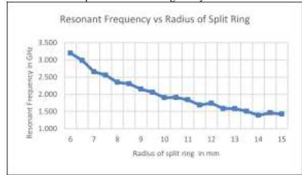
Figure 2b – Shift in resonant Frequency with variation in radius of SR
