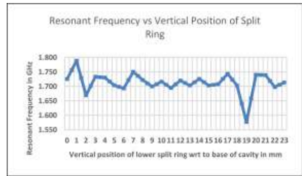
Figure 2a - Resonant frequency of single SSR with variation of vertical position of SR along cavity axis
