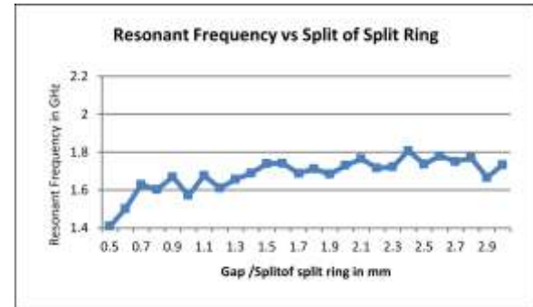
Figure 2c – Shift in resonant Frequency with variation in capacitive gap / split of SR
