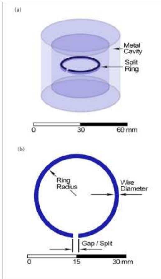
Figure 1 - Design structure for single SSR a) SSR within metallic cylindrical cavity (b) SR showing the gap/ split
