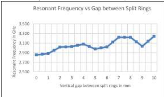
Figure 4b - Outer ring is moved upward in the cavity whereas inner ring is placed at 1 mm above base of cavity.
