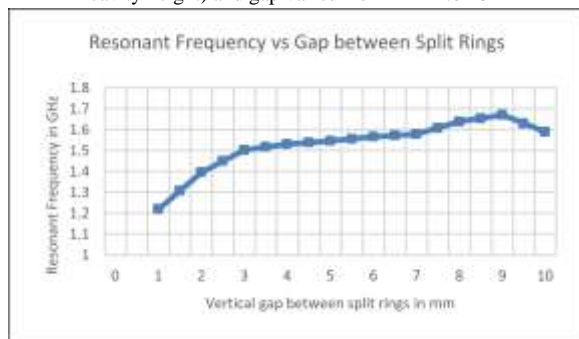
Figure 3b. Lower SR placed 1 mm above the base of cavity and gap varied from 1 mm to 10 mm
