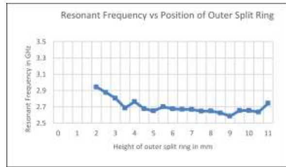
Figure 4c - Height of inner SR is fixed at 10 mm and outer split ring is moved up from lower position.
