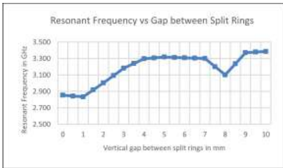
Figure 4a - Inner ring is moved upward in the cavity whereas outer ring is placed at 1 mm above base of cavity.
