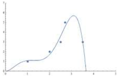
Figure 3. Smooth regression.
