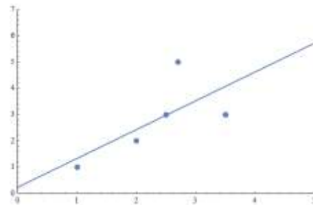
Figure 6. Underfitting effect.
