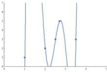
Figure 2. Overfitting effect.
