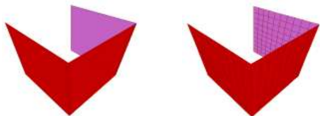
Figure 1. Shell element model and FEM of an U – Shaped shear wall
