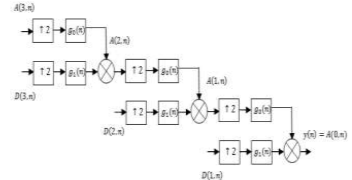
Figure.5. Three level resolution synthesis filter bank.
