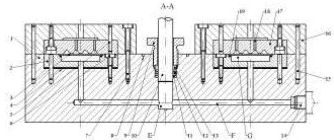
Figure 1. Principle of Multi-channel Sheet Hydroforming
