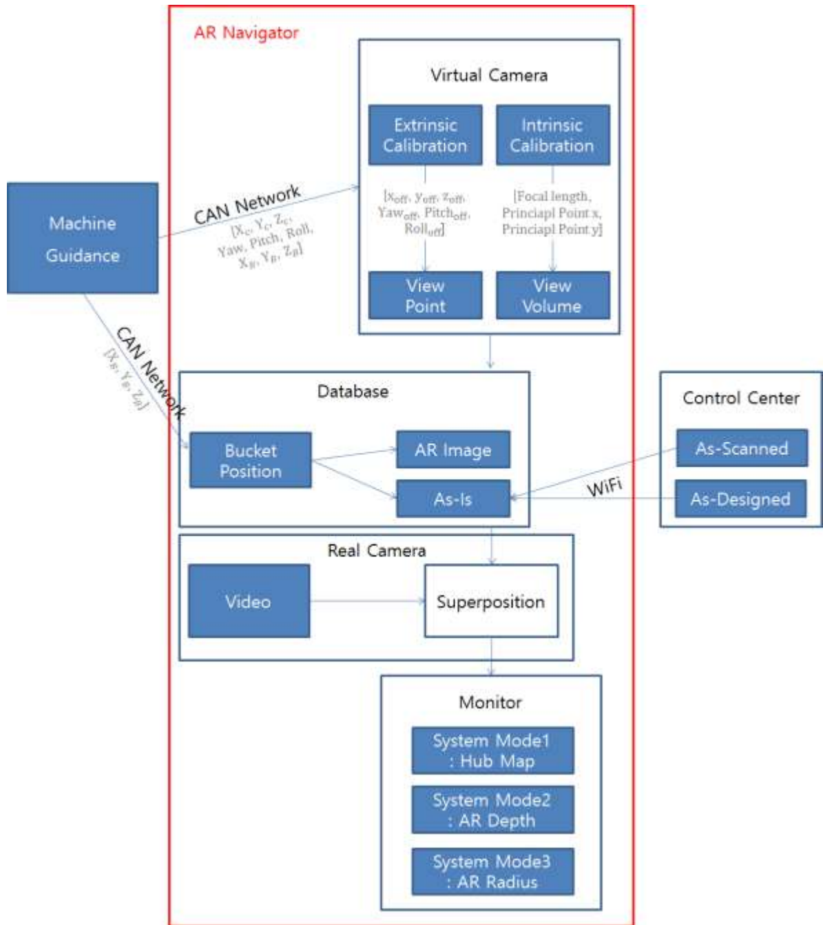
Figure 1. AR Navigator architecture
