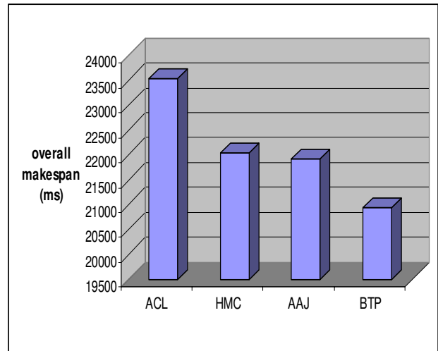
Figure 4. Overall Performance of different workload descriptor
