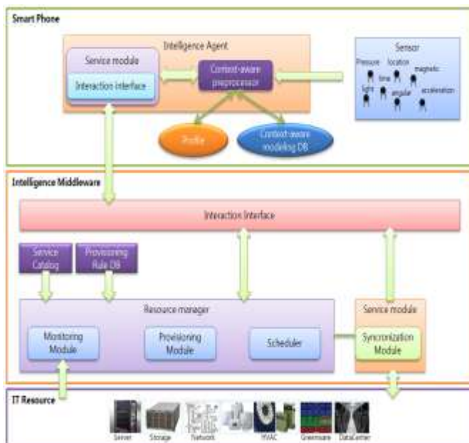
Fig. 1. Proposed Architecture
