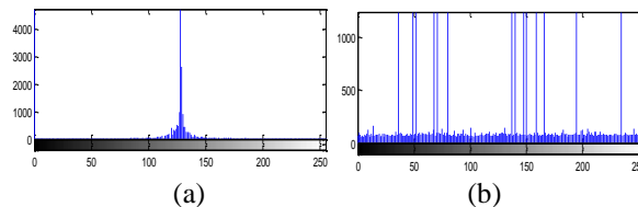
Figure 10. (a) Histogram of the original Speech quantized Image, (b) Histogram of the Encrypted Speech quantized Image.
