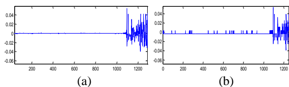
Figure 6. (a) The beginning of the original speech signal (Zoomed ), (b) the same region of the reconstructed speech signal after Decrypted and Dequantization (Zoomed).
