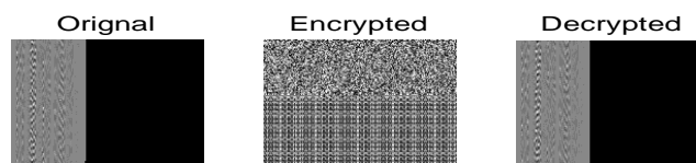
Figure 3. Image Encrypted/Decrypted.
