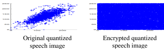
Figure 9. Correlation comparison.
