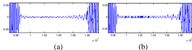
Figure 7. The middle of the original speech signal (Zoomed), (b) the same region of the reconstructed speech signal after Decrypted and Dequantization (Zoomed).
