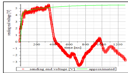
Fig.6 Characteristics impedance approximation
