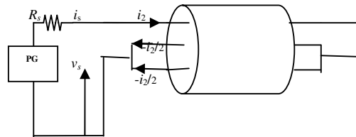
Fig.1 Test circuit for Mode 2
