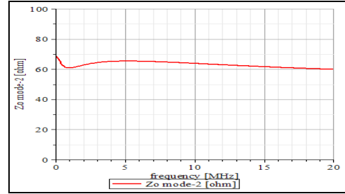
Fig.8 Characteristics impedance
