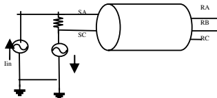
Fig. 4 EMTP branch card for mode-1 and mode-2
