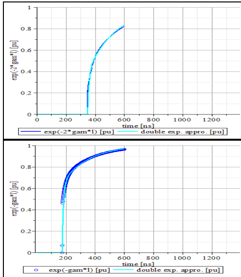
Fig.7 Wave propagation approximation
