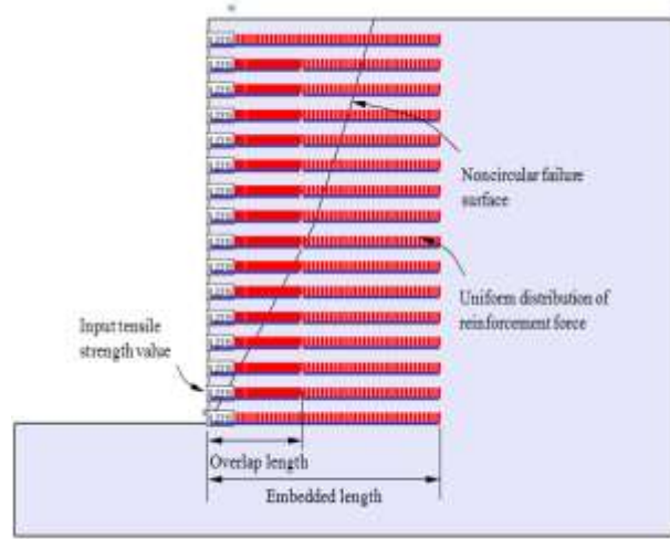
Figure 5. Reinforcement force distribution and failure surface used in LE analyses
