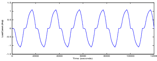
Figure 7. Load Current of 11-Level Inverter
