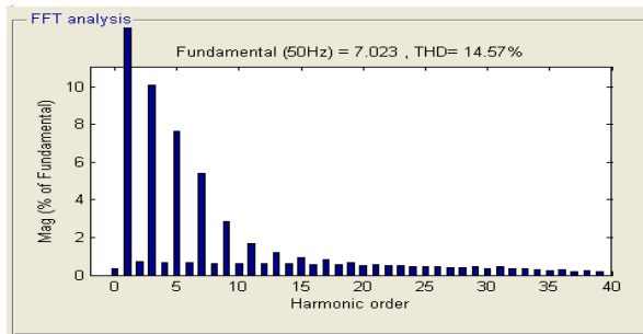
Figure 8. FFT Analysis of 7-Level Inverter
