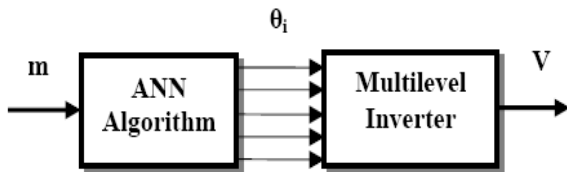
Figure 3. ANN Control of Inverter
