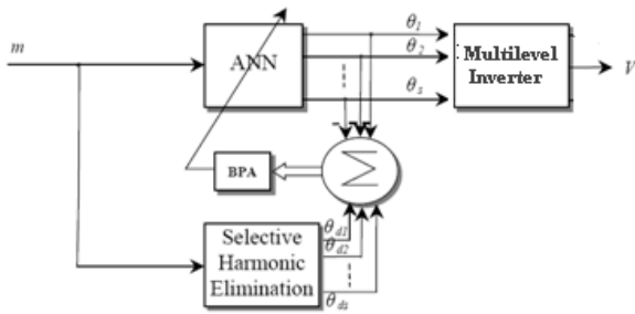
Figure 2. Back Propagation Algorithm
