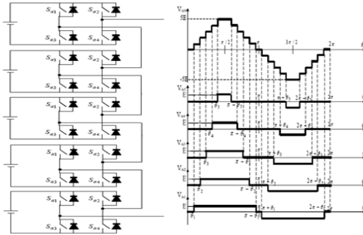
Figure 1. Multilevel Inverter and its Output Waveform
