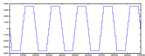
Figure 4. Output Voltage of 7-Level Inverter
