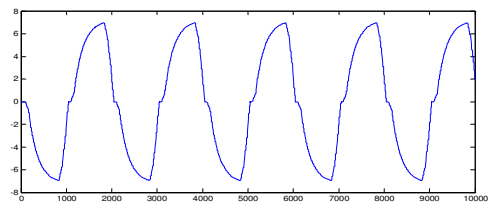
Figure 5. Load Current of 7-Level Inverter
