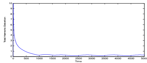
Figure 11. THD Analysis of 11-Level Inverter
