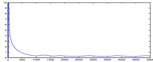
Figure 10. THD Analysis of 7-Level Inverter
