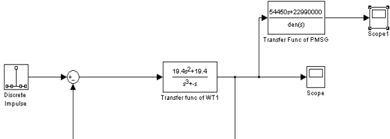
Figure 5. Wind Turbine driven PMSG in closed loop configuration.
