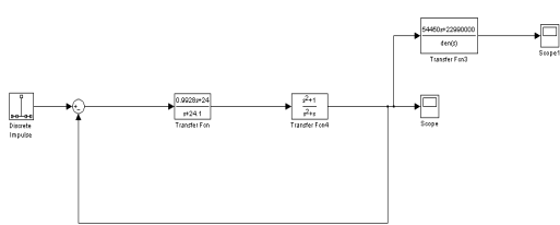
Figure 6. Wind Turbine driven PMSG in closed loop configuration with minimum order observer
