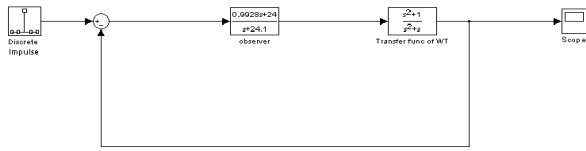
Figure 4. Closed loop configuration of the Wind Turbine with observer.
