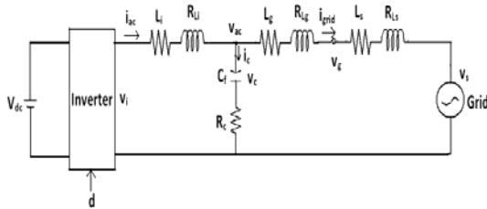
Fig ure 2. DC/AC inverter equivalent circuit
