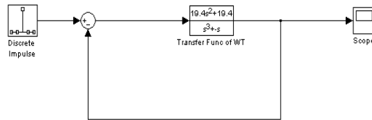
Figure 3. Wind Turbine in closed loop configuration
