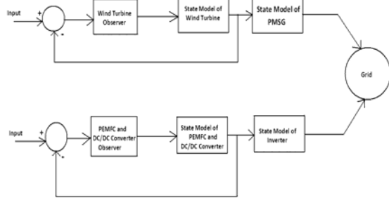
Figure 1. Grid integrated system with the implementation of minimum order observer.
