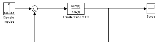
Figure 7. Simulink circuit of the model of fuel cell in closed loop configuration.
