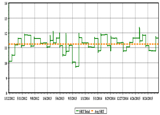
Fig. 8: Predicted SRT for the period 2012 to 2015: FSTW Unit 4
