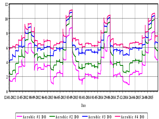
Fig. 9: Predicted DO concentrations in the aeration zone FSTW Unit 4: 2012 to 2015
