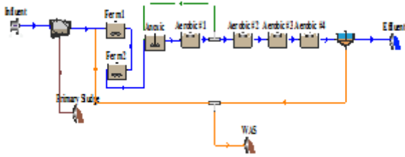
Fig. 2: BioWin Abstract Process Flow Diagram (PFD): FSTW Unit 4 (see study design for rational of aeration divisions)
