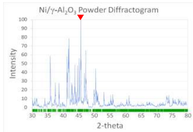
Figure 3a. Calculated Diffractogram for Ni/γ-Al 2 O 3
