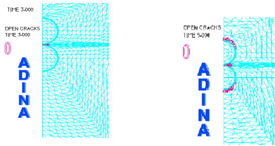
(a) Time increment 3. (b) : Time increment 5. Figure 6: Temperature producing first radial cracks in concrete at FRP bar/concrete interface for the beam P.#13.20: (a) in bars interaction zone, (b) in FRP bar/concrete interface zone.
