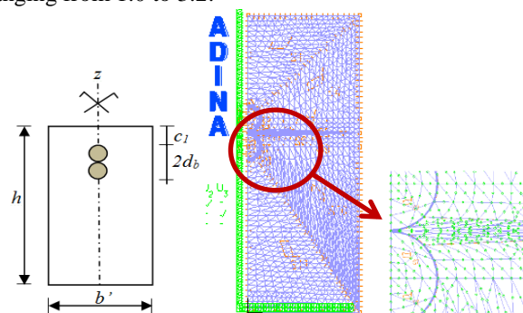
Figure 1. Geometry and mesh diagram of a cross section of concrete beam reinforced with two GFRP bars.
