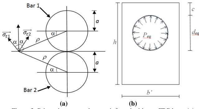
Figure 3: Prismatic concrete beam reinforced with two FRP bars: (a) Schema of the overlapped bars stresses. (b) The cross section replacing the overlapped bars section by one equivalent FRP bar section.
