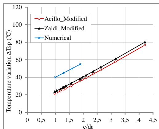
Figure 7: Temperature variations producing the total failure of concrete cover ( \Delta T_{sp} ) for concrete beams reinforced with two overlapped bars.
