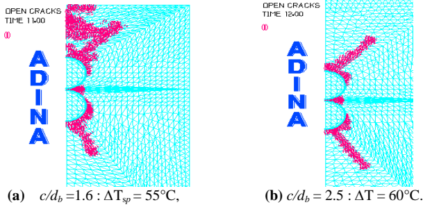
Figure 8: Cracks propagation in concrete cover: (a) Total Cracking of concrete cover of beam P.#13.20 (b) Partial cracking of beam P.#13.30.
