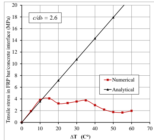
Figure 9: Transverse tensile stress in concrete at FRP bar/concrete interface of beam for beam P.#25.10, having c/d_b=2.6 .
