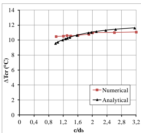
Figure 5: Temperature variation producing the first radial crack in concrete at FRP bar/concrete interface of beams reinforced with two overlapped bars.
