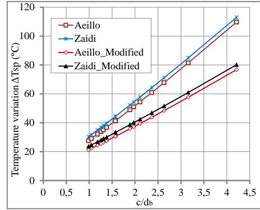
Figure 4. Temperature variations producing a total failure of concrete cover of overlapped and non-overlapped bars sections.
