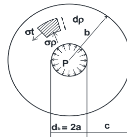
Figure 2. Concrete cylinder concentrically reinforced with FRP bar.
