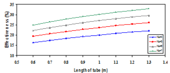
Figure 2. Variation of efficiency on heat pipe and the number of rows
