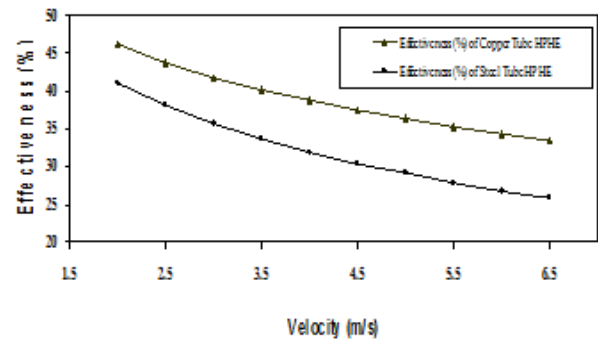
Figure 1. Variation efficiency than velocity in copper and steel heat pipe
