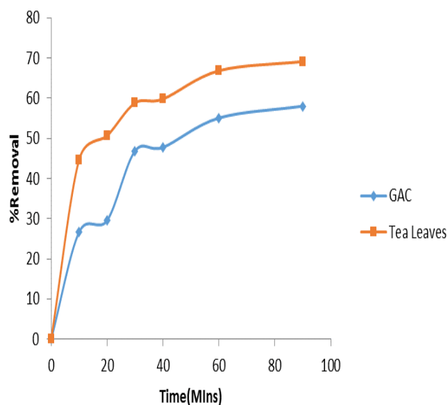
Figure 2: Plot of % removal of progesterone by tea leaves and GAC at pH 7, temperature 25°C
