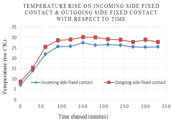
Fig. 11 Variation of Temperature rise with time for Incoming & Outgoing contacts of fixed assembly of 220 kV isolator
