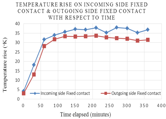
Fig. 8 Variation of Temperature rise with time for Incoming & Outgoing side fixed contact of 66 kV isolator
