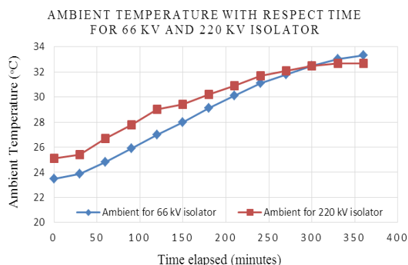
Fig. 13 Variation of Ambient Temperature with period during current energisation of sample.
