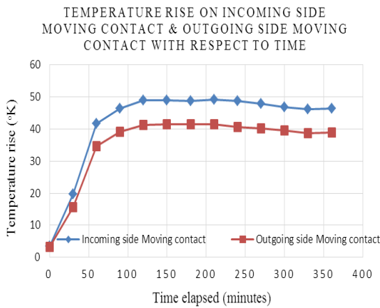
Fig. 9 Variation of Temperature rise with time for Incoming & Outgoing side moving contact of 66 kV isolator
