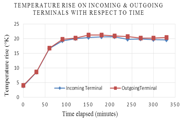
Fig. 10 Variation of Temperature rise with time elapsed for Incoming & Outgoing terminals of 220 kV Isolator
