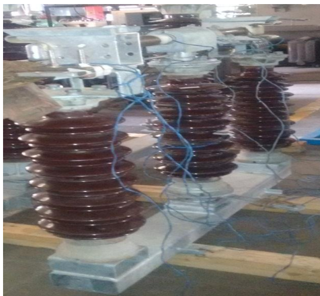
Fig. 1 Experimental arrangement for 66 kV Isolator with central break system
