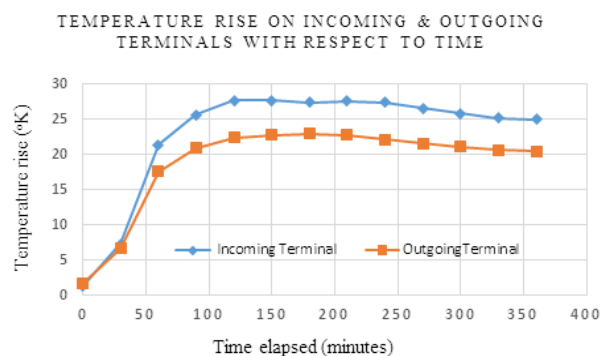
Fig. 7 Variation of Temperature rise with time elapsed for Incoming & Outgoing terminals of 66 kV isolator
