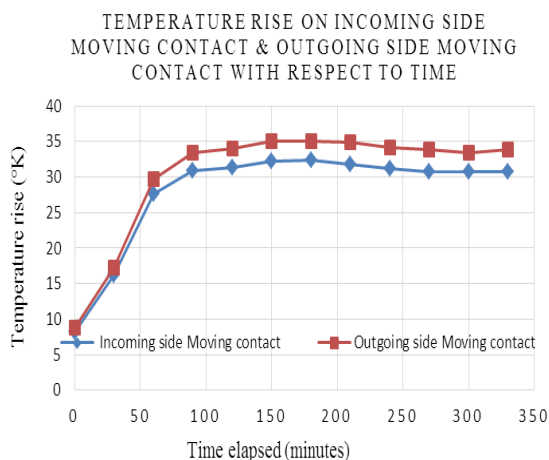
Fig. 12 Variation of Temperature rise with duration for Incoming & Outgoing side Moving Contact of 220 kV Isolator
