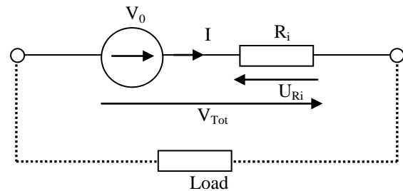
Figure 2. Electrical schema of nanogenerator.
