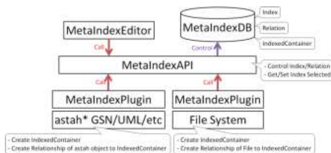
Figure 2 Block diagram of MetaIndexTools
