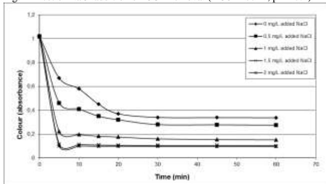
Fig.3 Effect of NaCl addition on colour removal (I=50mA/cm 2 , pH= 7.2)
