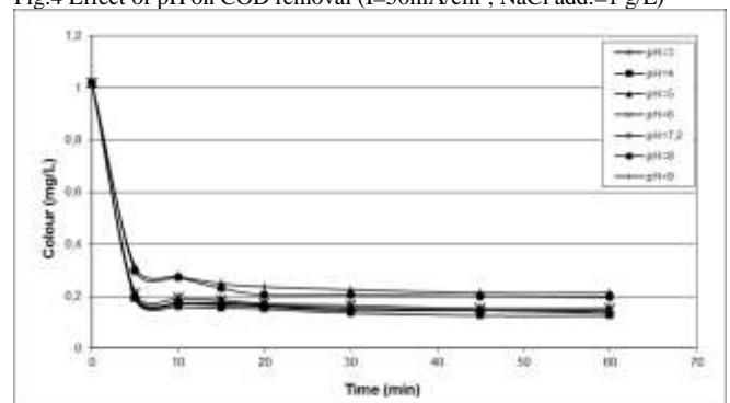
Fig.5 Effect of pH on colour removal (I=50mA/cm 2 , NaCl add.=1 g/L)
