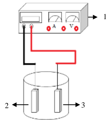
Figure 1. Experimental setup used in electrochemical ozone generation: (1) power supply (2)anode, (3) cathode
