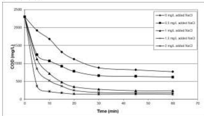
Fig.2 Effect of NaCl addition on COD removal (I=50mA/cm 2 , pH= 7.2)
