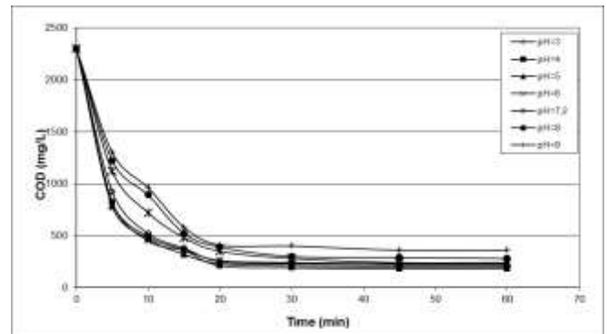
Fig.4 Effect of pH on COD removal (I=50mA/cm 2 , NaCl add.=1 g/L)
