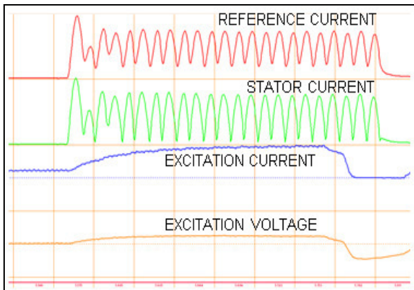
Fig-7. Waveforms during Generator Mode.
