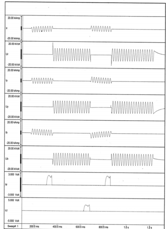
Fig.9. Duty cycle on a Circuit Breaker.
