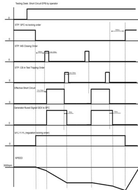
Fig.5: Chronograms of SC Test sequence.
