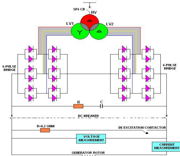
Fig-2 Single Line Diagram of GEX.
