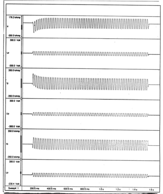
Fig.8. Long duration Test on CT.
