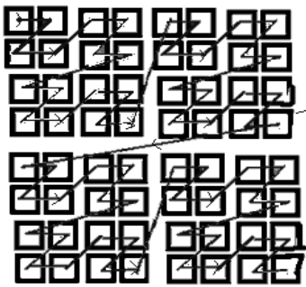
Figure 5. Figure showing scanning order for a 8x8 image. The scanning begins in the order : LL3,HL3,LH3,HH3,HL2,LH2,HH2,HL1,LH1 & HH1. The scanning order continues in the direction of arrow known as Morton scanning.
