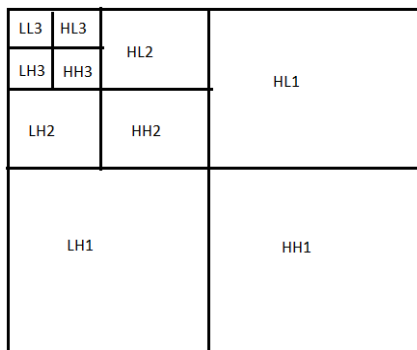
Figure 2. Figure showing the three levels of wavelet decomposition. The third decomposition level is obtained by further decomposition of LL2 sub-band. This decomposition clusters the maximum energy in the LL3 sub-band.
