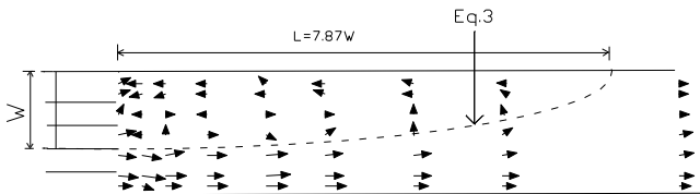
Fig. 9a Distribution of velocity vectors for e=3.5 , H_u/G=5.00 , and Y_t/Y_3=1.40 at 0.5Y .
