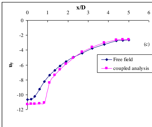
Fig. 2 Ground surface displacements for free field and coupled analyses (a) x direction; b) z direction; and c) y direction.
