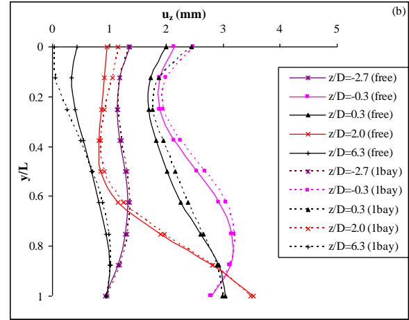
Fig. 5 Influence of super-structure interaction on piles' longitudinal deformation ( u_z ) during tunnelling for one bay structure: a) P1; b) P2
