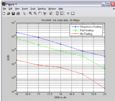
Figure 7: 16-QAM ,3/4 code rate, 36 Mbps
