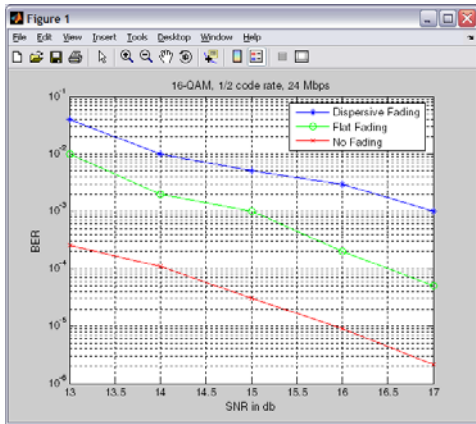
Figure 6: 16-QAM ,1/2 code rate, 24 Mbps
