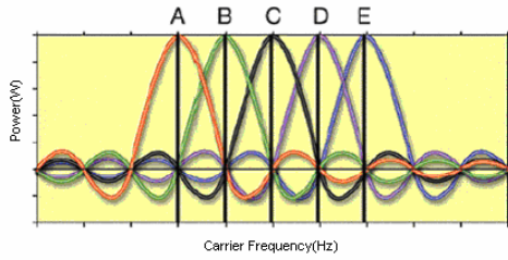
Figure 1.Orthogonally overlapped subcarriers
