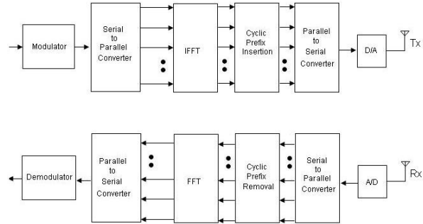
Figure 3.Ofdm transceiver
