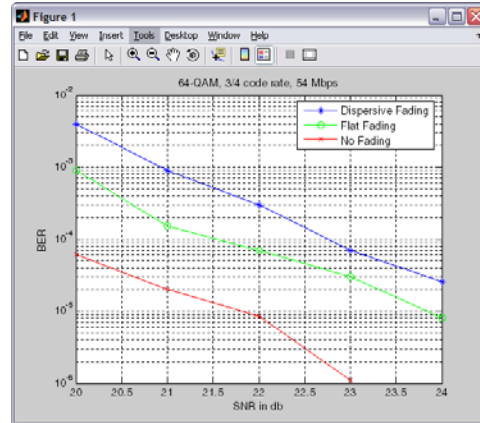
Figure 9: 64-QAM ,3/4 code rate, 54 Mbps
