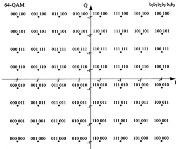
Figure 5. 64-QAM constellation points
