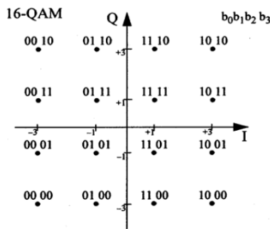
Figure 4. 16-QAM constellation points
