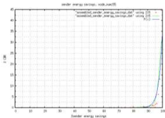
Figure 49: % cbr for SES node_number 55 50. Node Number 56
