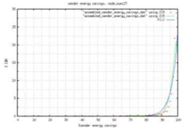
Figure 21: % cbr for SES node_number 27
