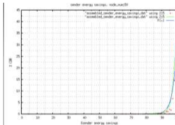
Figure 44: % cbr for SES node_number 50 45. Node Number 51
