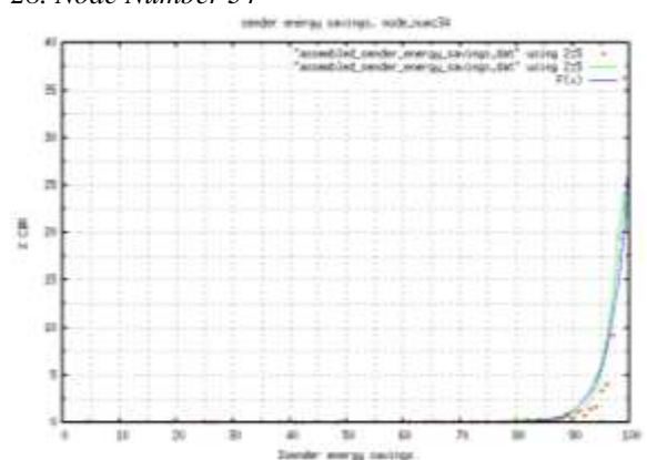
Figure 28: % cbr for SES node_number 34 29. Node Number 35
