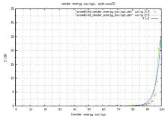
Figure 26: % cbr for SES node_number 32 27. Node Number 33
