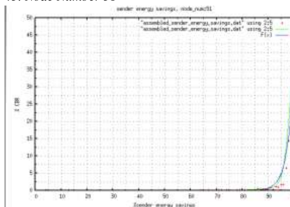
Figure 45: % cbr for SES node_number 51 46. Node Number 52
