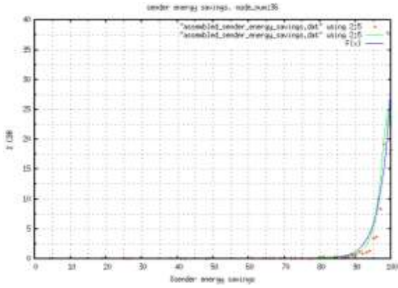
Figure 30: % cbr for SES node_number 36 31. Node Number 37
