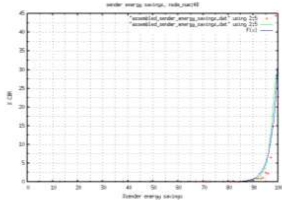
Figure 42: % cbr for SES node_number 48 43. Node Number 49
