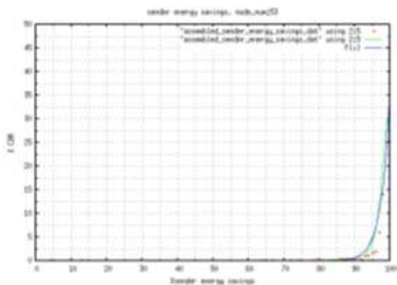
Figure 47: % cbr for SES node_number 53 48. Node Number 54
