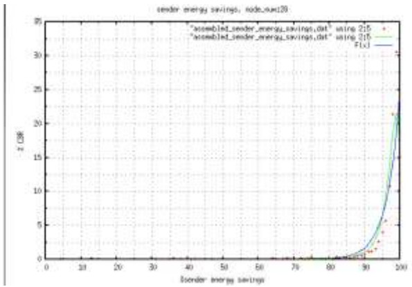
Figure 22: % cbr for SES node_number 28 23. Node Number 29
