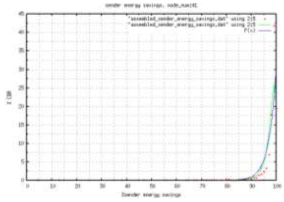
Figure 35: % cbr for SES node_number 41 36. Node Number 42
