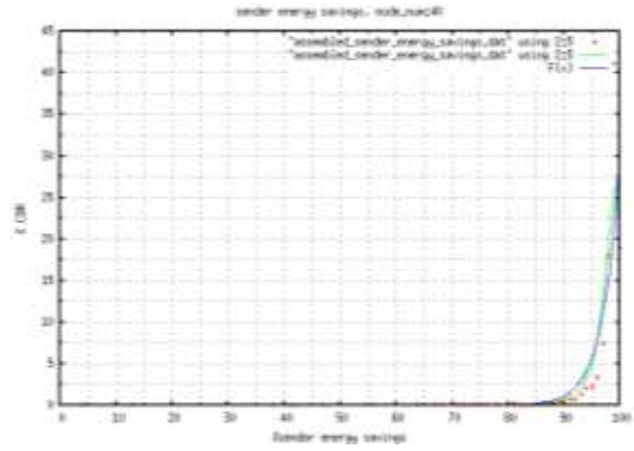
Figure 34: % cbr for SES node_number 40 35. Node Number 41
