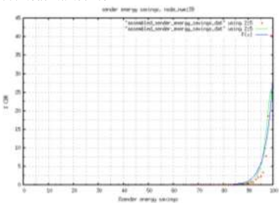
Figure 33: % cbr for SES node_number 39 34. Node Number 40
