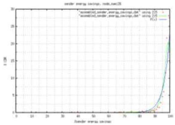
Figure 20: % cbr for SES node_number 26
