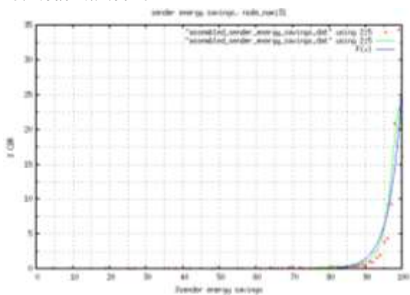
Figure 25: % cbr for SES node_number 31 26. Node Number 32
