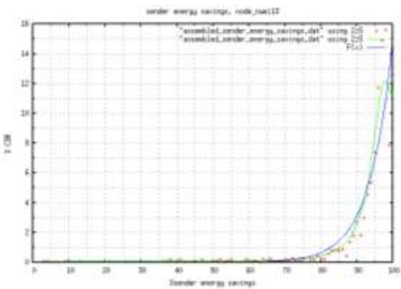
Figure 7: % cbr for SES node_number 13 8. Node Number 14
