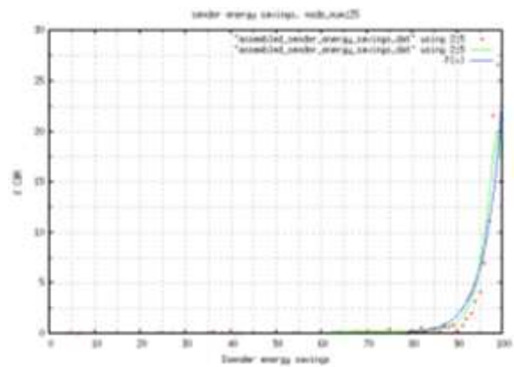
Figure 19: % cbr for SES node_number 25
