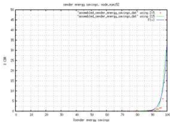
Figure 46: % cbr for SES node_number 52 47. Node Number 53
