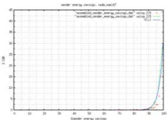
Figure 41: % cbr for SES node_number 47 42. Node Number 48
