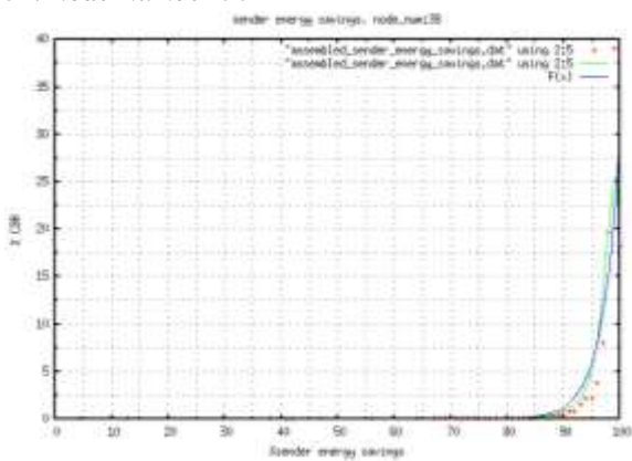
Figure 32: % cbr for SES node_number 38 33. Node Number 39
