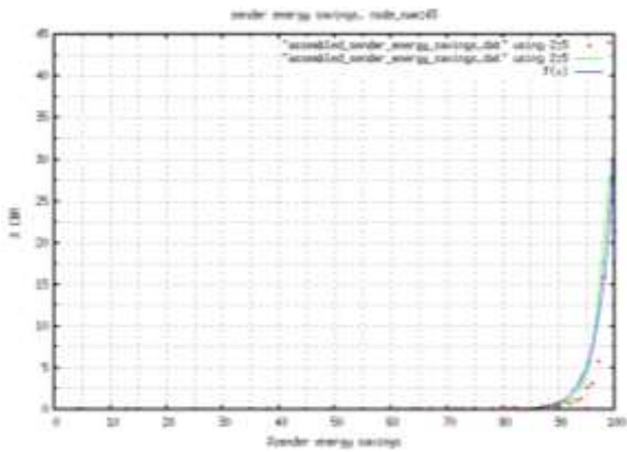
Figure 39: % cbr for SES node_number 45 40. Node Number 46
