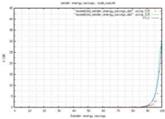
Figure 38: % cbr for SES node_number 44 39. Node Number 45
