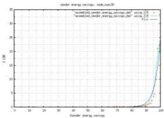
Figure 24: % cbr for SES node_number 30 25. Node Number 31
