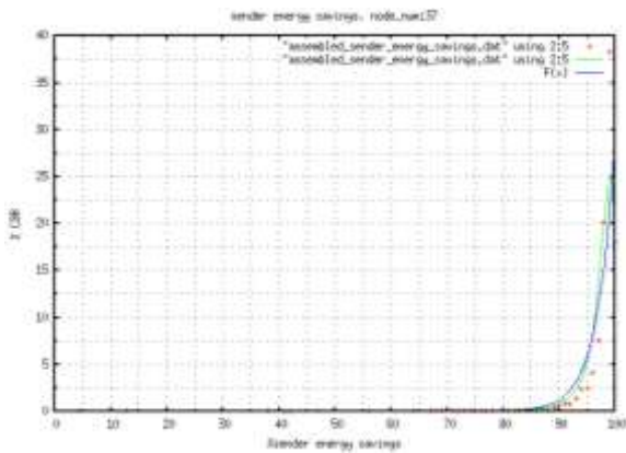
Figure 31: % cbr for SES node_number 37 32. Node Number 38
