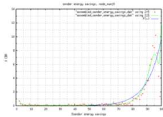
Figure 3: % cbr for SES node_number 9
