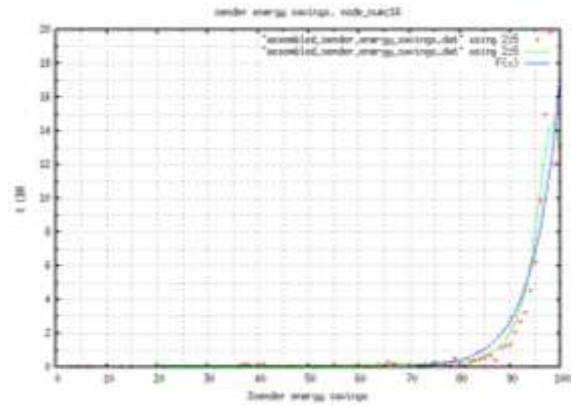
Figure 10: % cbr for SES node_number 16 11. Node Number 17
