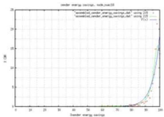
Figure 12: % cbr for SES node_number 18 13. Node Number 19
