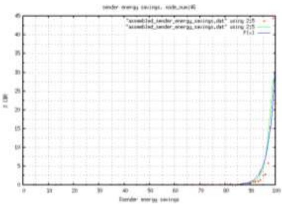
Figure 40: % cbr for SES node_number 46 41. Node Number 47
