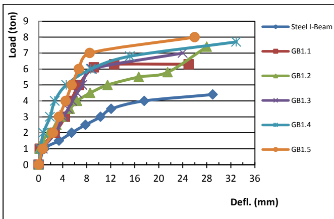
Figure (12): Load Deflection Curves at mid span (group 1)
