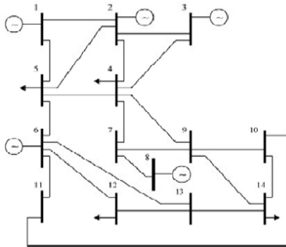
2. single line diagram of 14 bus IEEE network
