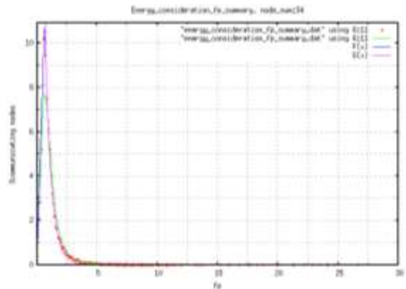
Figure 28: % communicating nodes for ECFP node_number 34 29. Node Number 35
