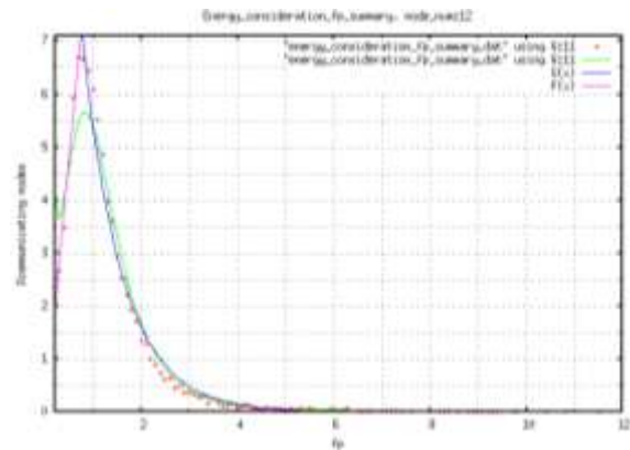
Figure 6: % communicating nodes for ECFP node_number 12 7. Node Number 13
