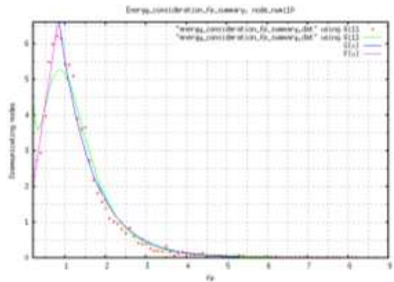
Figure 4: % communicating nodes for ECFP node_number 10 5. Node Number 11
