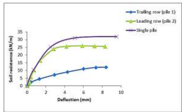
Figure 8. p-y curves [(2x2) group, S=2D, depth= 1.5 m]
