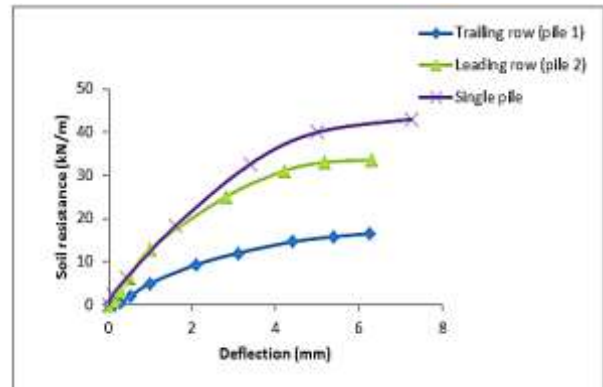
Figure 9. p-y curves [(2x2) group, S=2D, depth= 3.0 m]
