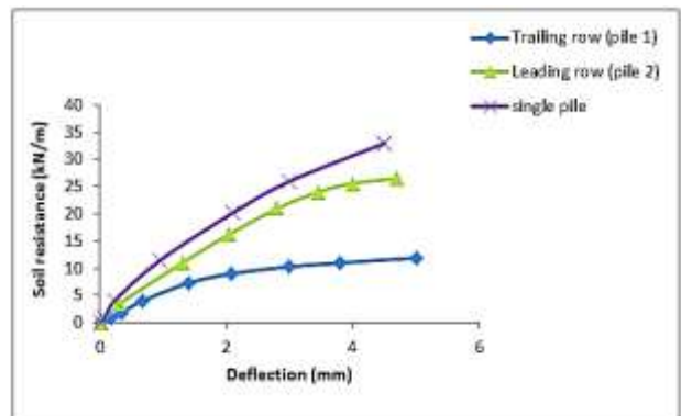
Figure 10. p-y curves [(2x2) group, S=7D, depth= 4.5 m]
