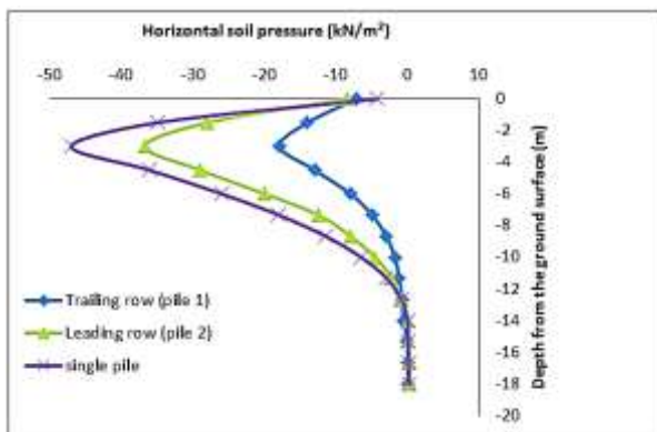
Figure 7. Horizontal soil pressure [(2x2) group, S=2D, max. displacement = 12.7 mm]
