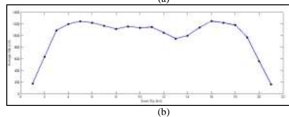
Figure 7. Variation of displacement at dip of 10 km along the fault (a) Five samples obtained from the source dimension (Wells and Coppersmith, 1994), (b) Average of five samples
