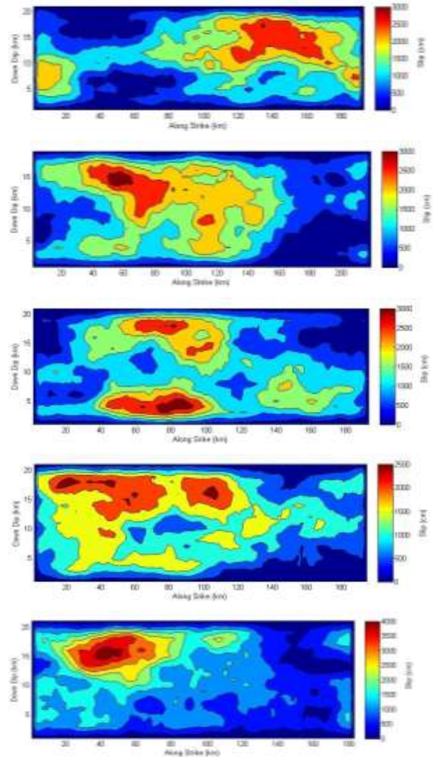
Figure 2 Sample slip field on rupture plane for 1934 Bihar-Nepal earthquake, Mw 8.1 (Mai and Beroza, 2000)
