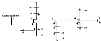
Figure 2. IEEE 15-Bus Test System
