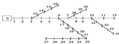
Figure 3. IEEE 34-Bus Test System
