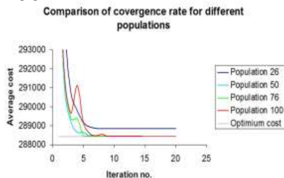
Figure 5: Comparison of convergence rate for different population.
