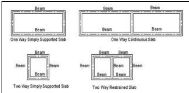
Fig1: Types of R.C.C. Slabs
