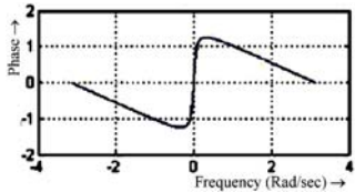
Figure 6. Phase v/s Frequency plot of Pre-emphasis Filter
