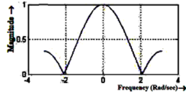
Figure 3. Magnitude v/s Frequency plot of moving average filter
