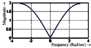
Figure 5. Magnitude v/s Frequency plot of Pre-emphasis Filter
