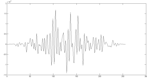
Figure 8. A Windowed Signal
